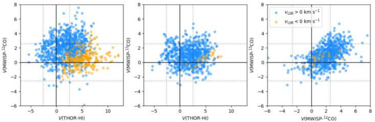
Fig. 3. Comparison between the values of the projected Rayleigh statistic ( V ) in the THOR HI and the MWISP CO observations. The two colors correspond to the positive and negative radial velocities. The dotted lines mark the 3\sigma significance thresholds in V .
